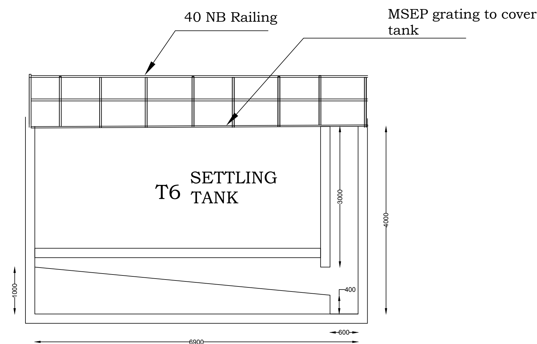
SECTION B-B
